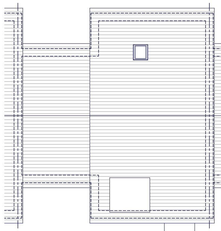
ROOF PLAN
