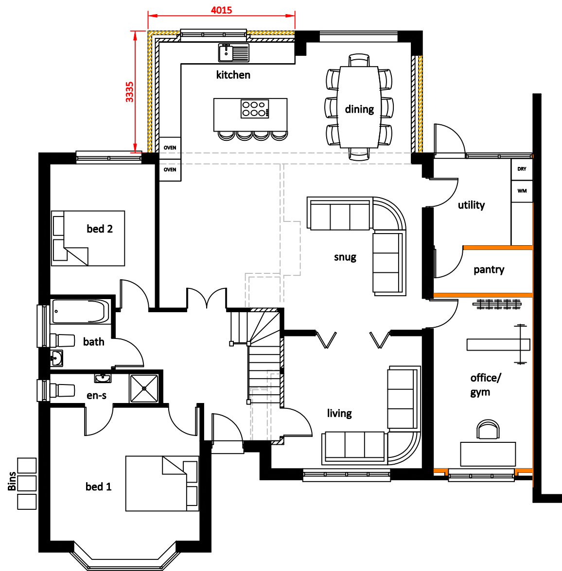
Ground 1:100
