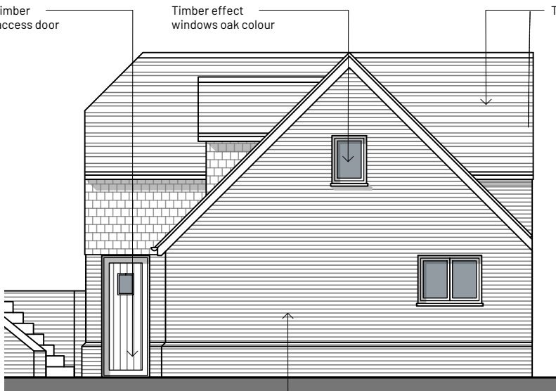
● SIDE ELEVATION (SOUTH FACING)
