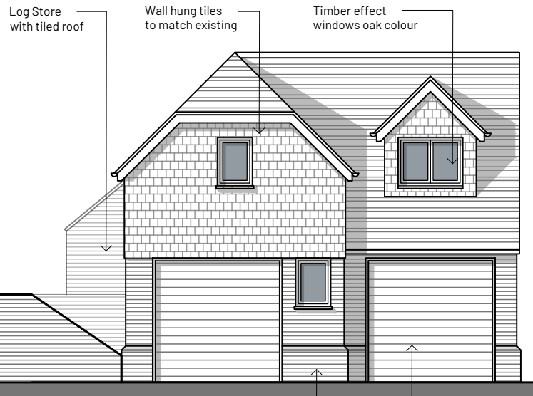
● FRONT ELEVATION (WEST FACING)
