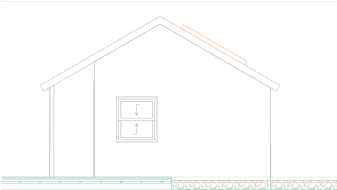
CLUBHOUSE NORTH ELEVATION - PROPOSED
