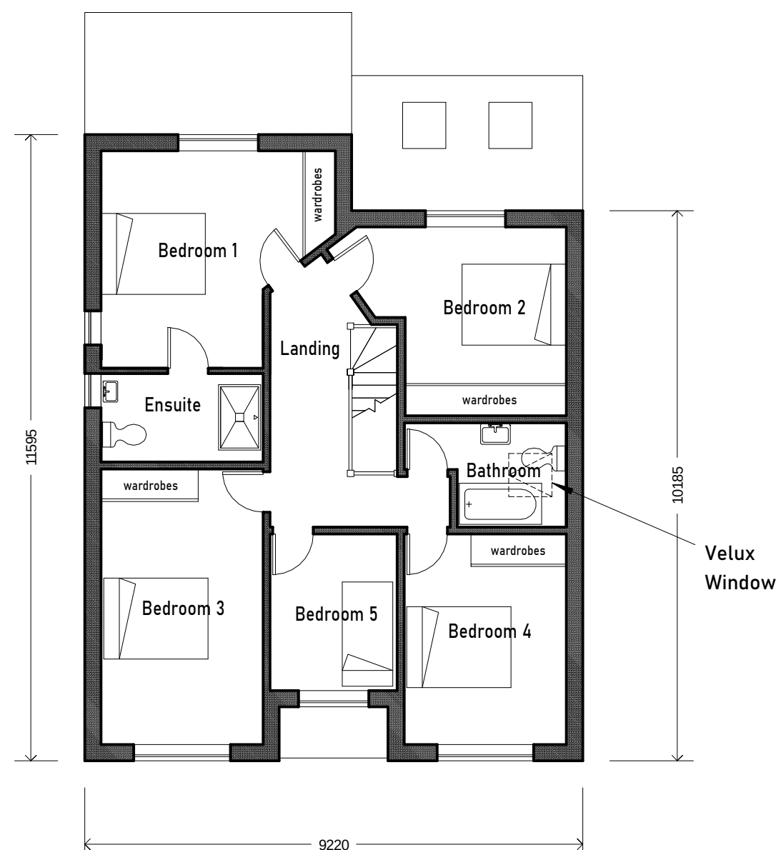
FIRST FLOOR
