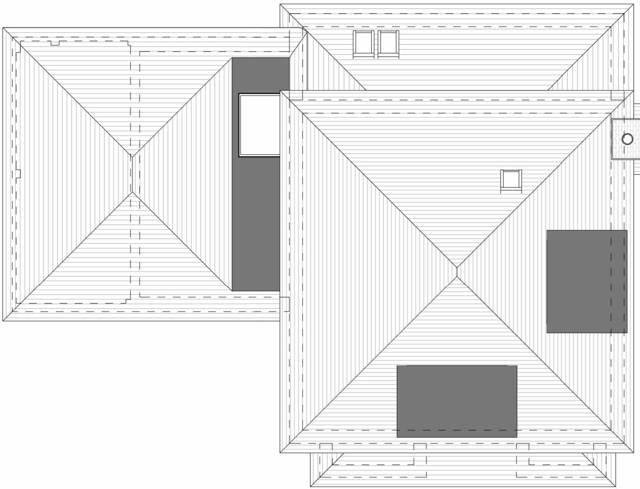
ROOF PLAN
