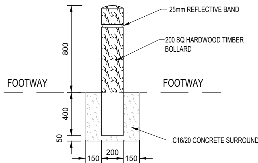
CYCLEWAY BOLLARD DETAIL
