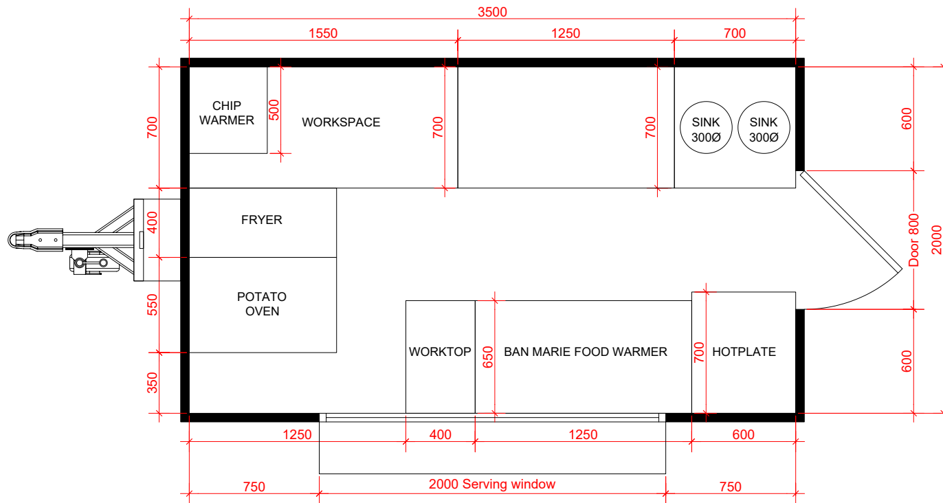
Floorplan
