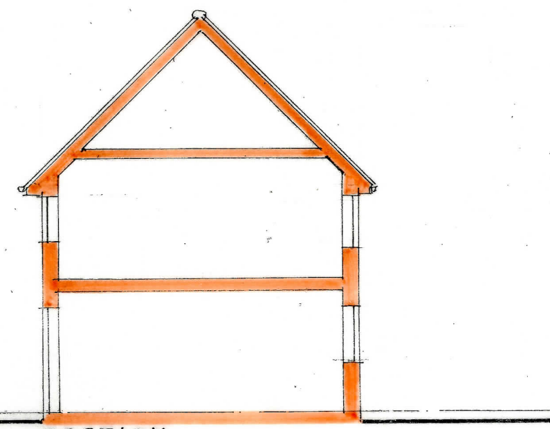
SECTION
