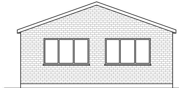
Proposed South Elevation
