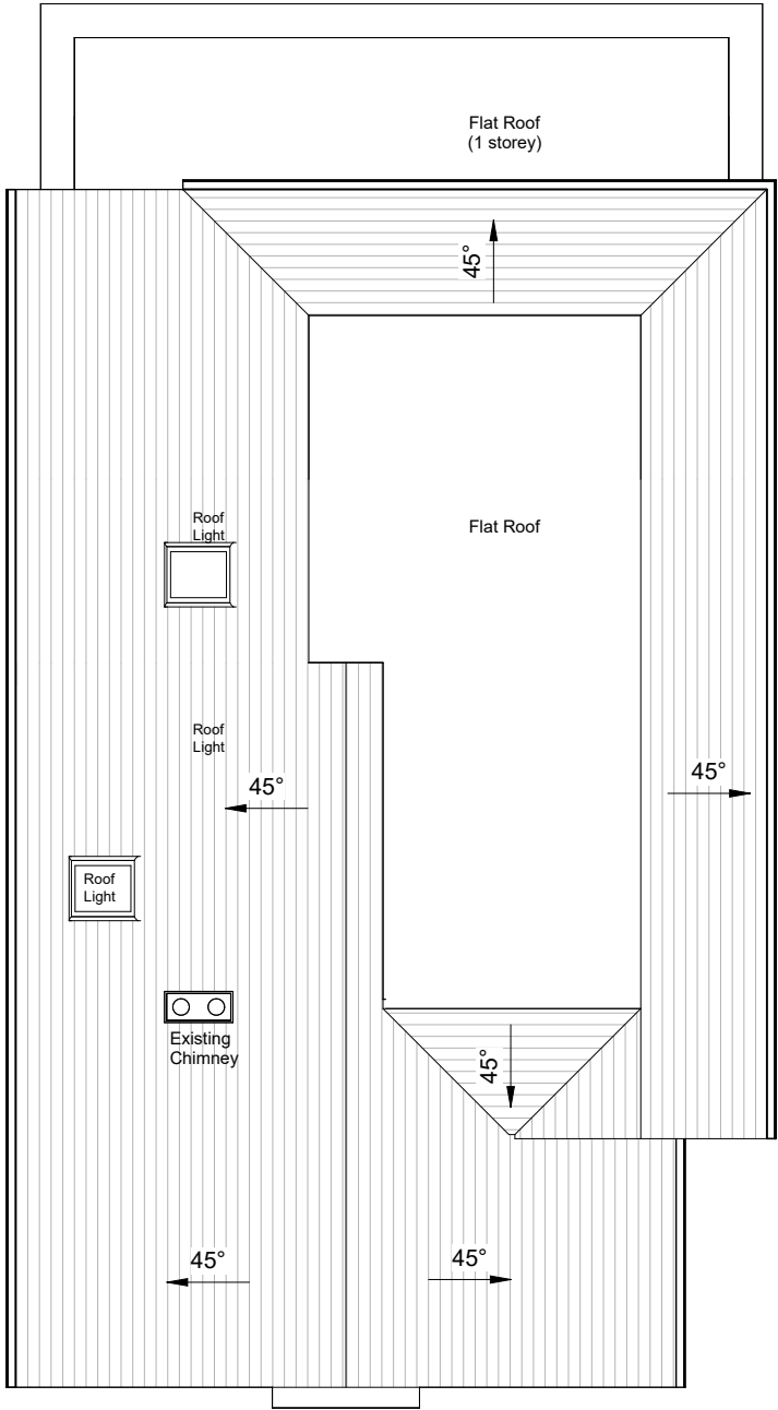
1 Proposed Roof Plan 1 : 100
