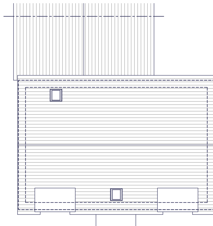
ROOF PLAN
