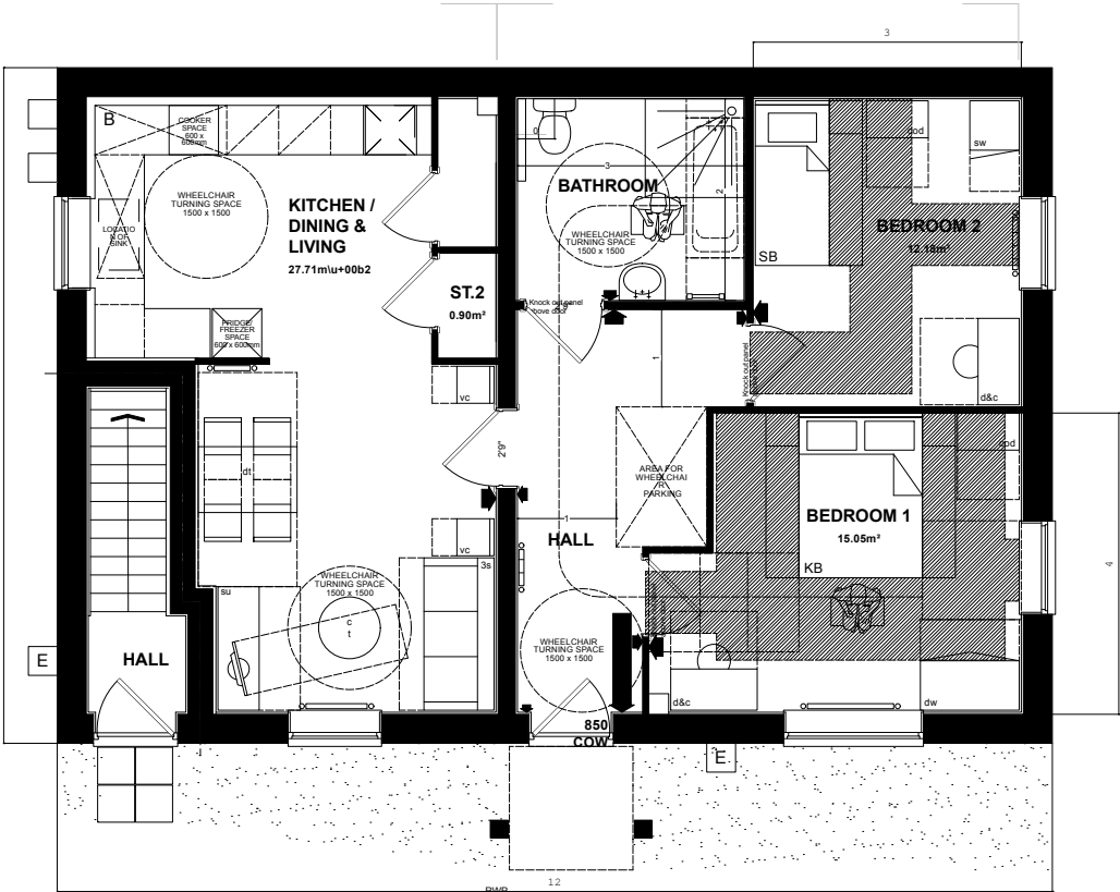
NSS.M(3)2BF03 GROUND FLOOR PLAN
