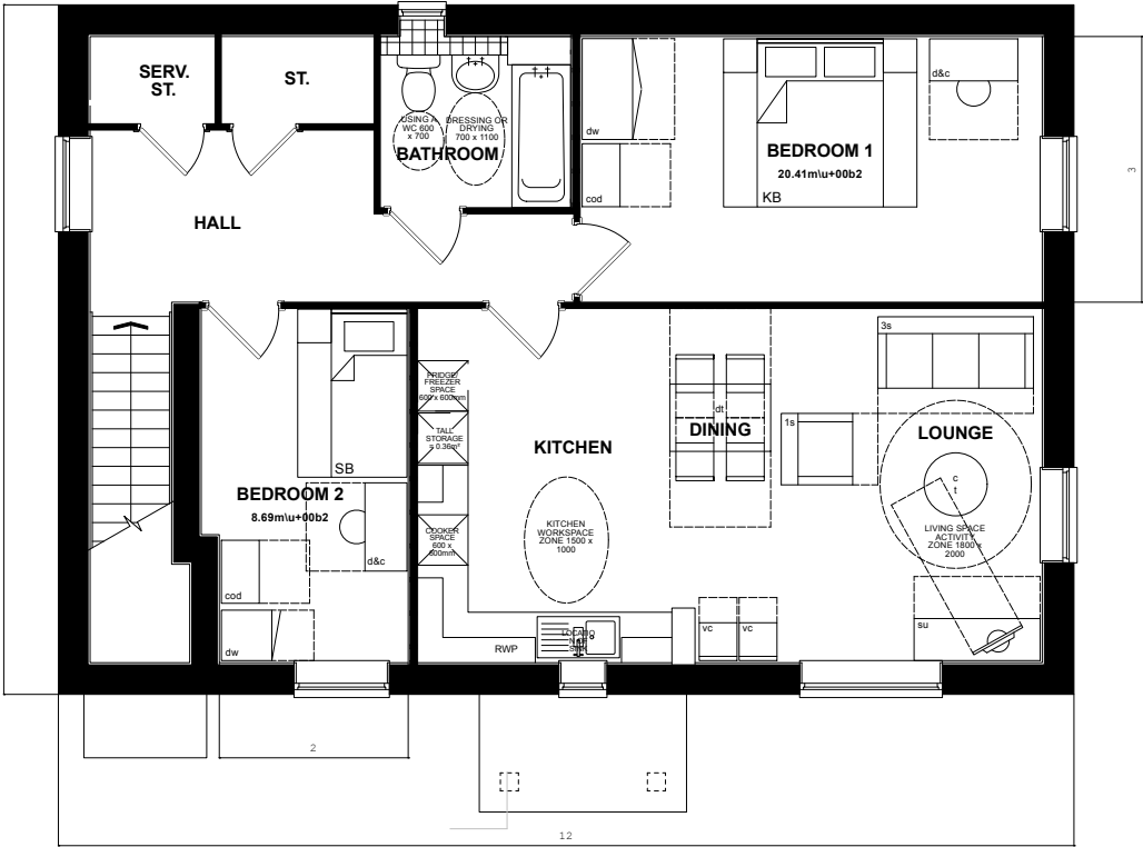
NSS.2BF03 FIRST FLOOR PLAN
