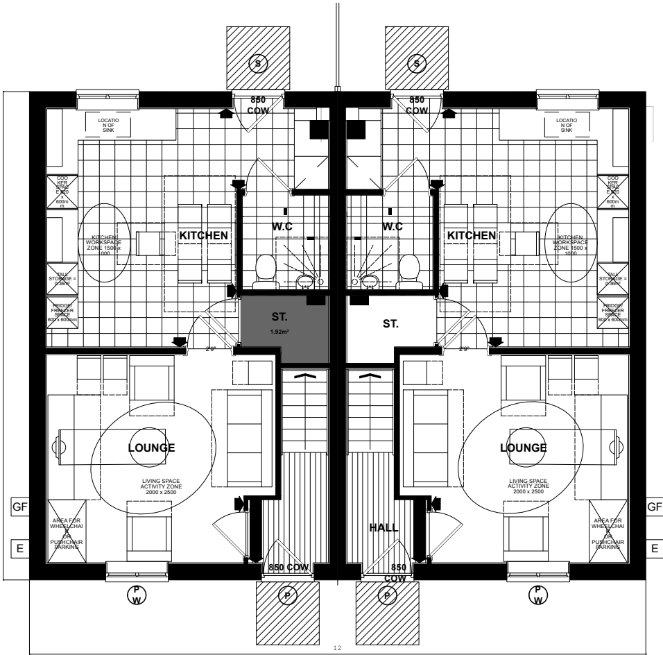
NSS.M3B5P GROUND FLOOR PLAN
