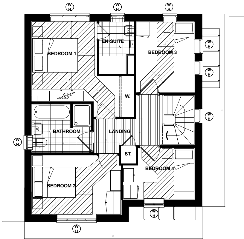
M401 FIRST FLOOR PLAN
