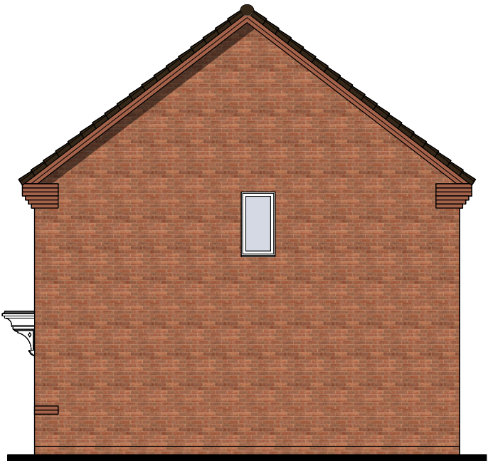
SIDE ELEVATION
