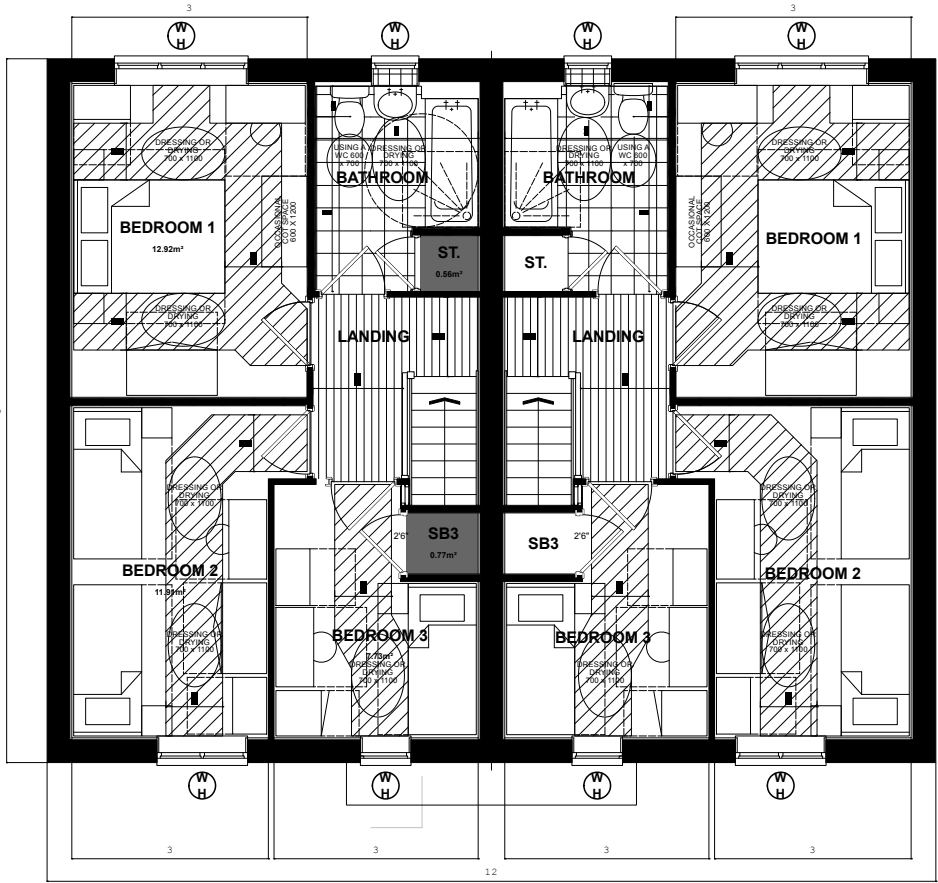
NSS.M3B5P FIRST FLOOR PLAN
