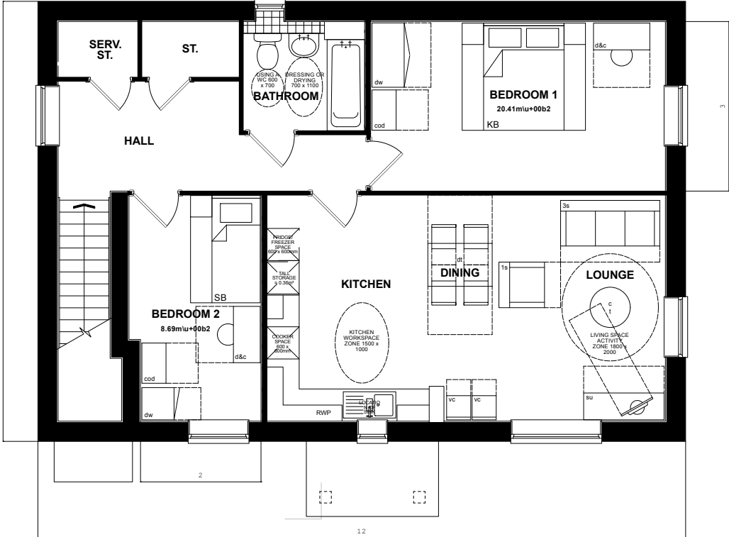
NSS.2BF03 FIRST FLOOR PLAN
