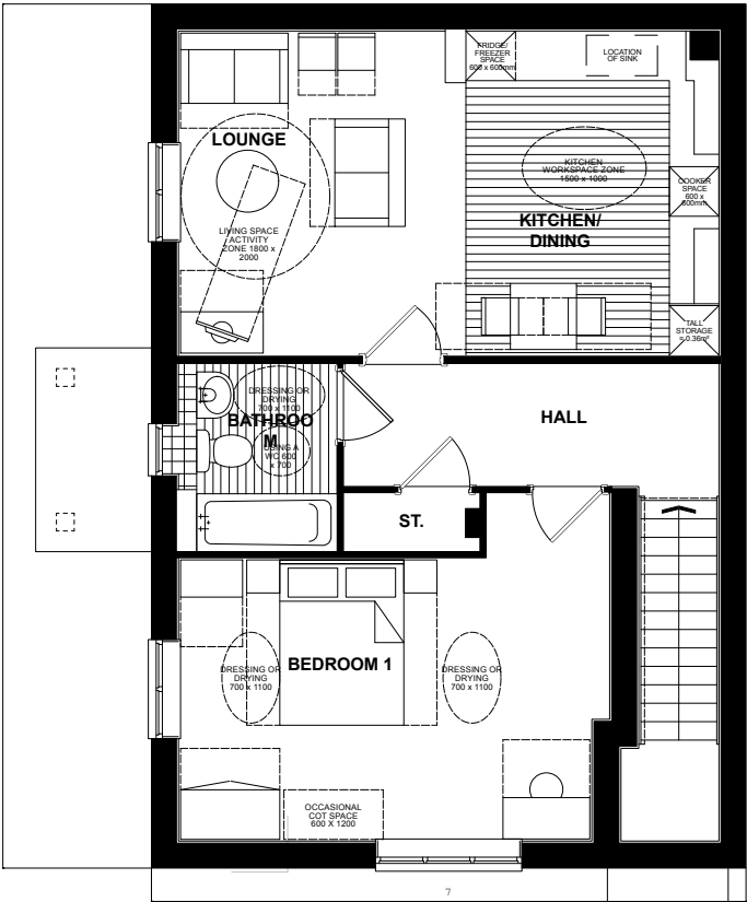
M4(3)1BF01 FIRST FLOOR PLAN
