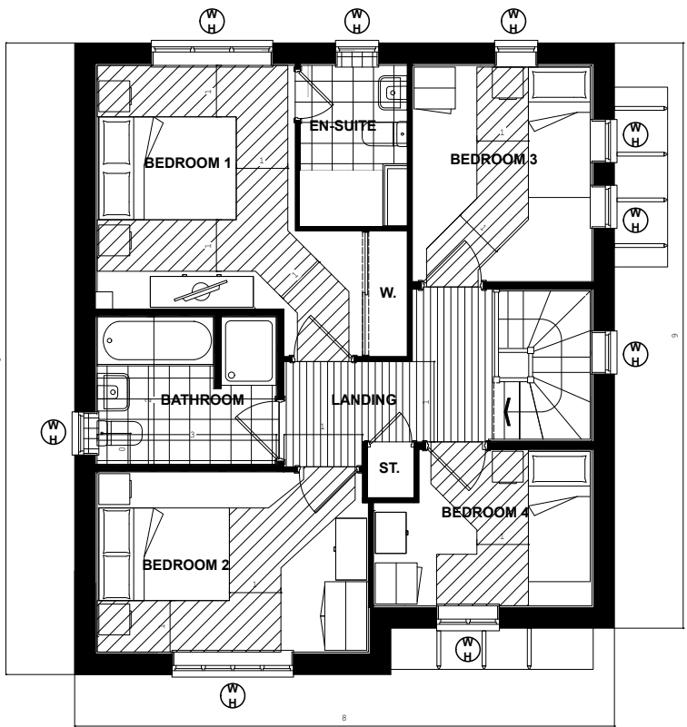
M401 FIRST FLOOR PLAN
