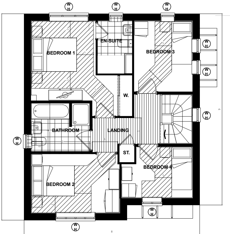
M401 FIRST FLOOR PLAN
