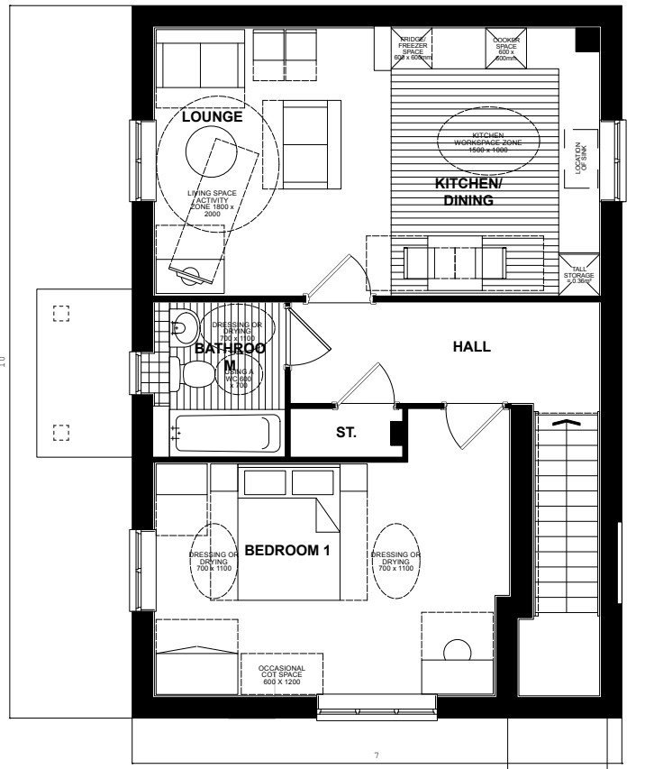
M4(3)1BF01 FIRST FLOOR PLAN
