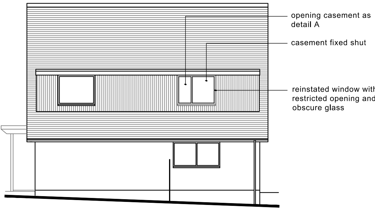
W. Side Elevation 1:100
