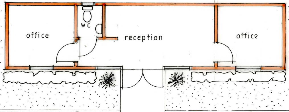
FLOOR PLAN
