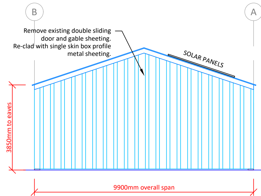
ELEVATION ACROSS GRIDLINE 10
