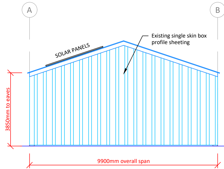
ELEVATION ACROSS GRIDLINE 1
