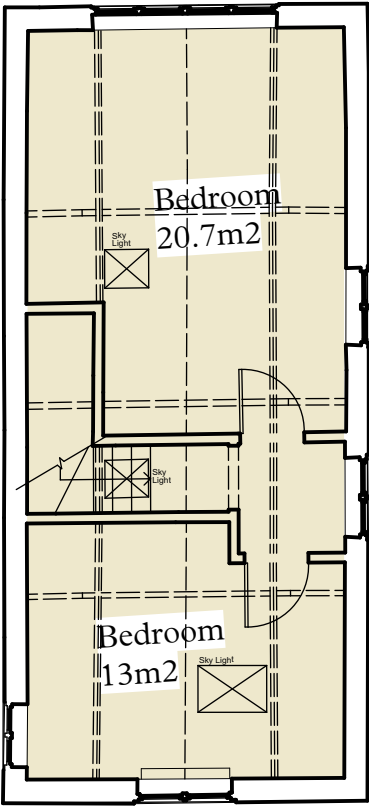
Coach House First Floor Plan GIA 42m2 GEA 50.66m2
