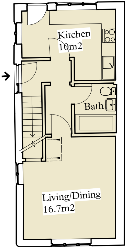
Coach House Ground Floor Plan GIA 40m2 GEA 50.07m2
