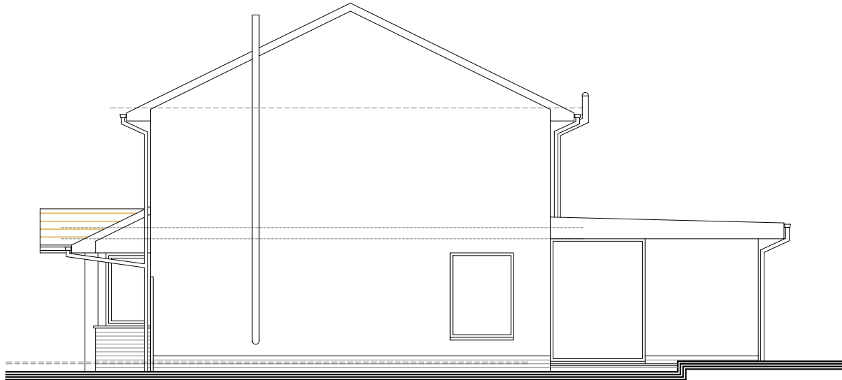
1:100 Existing Rh side Elevation
