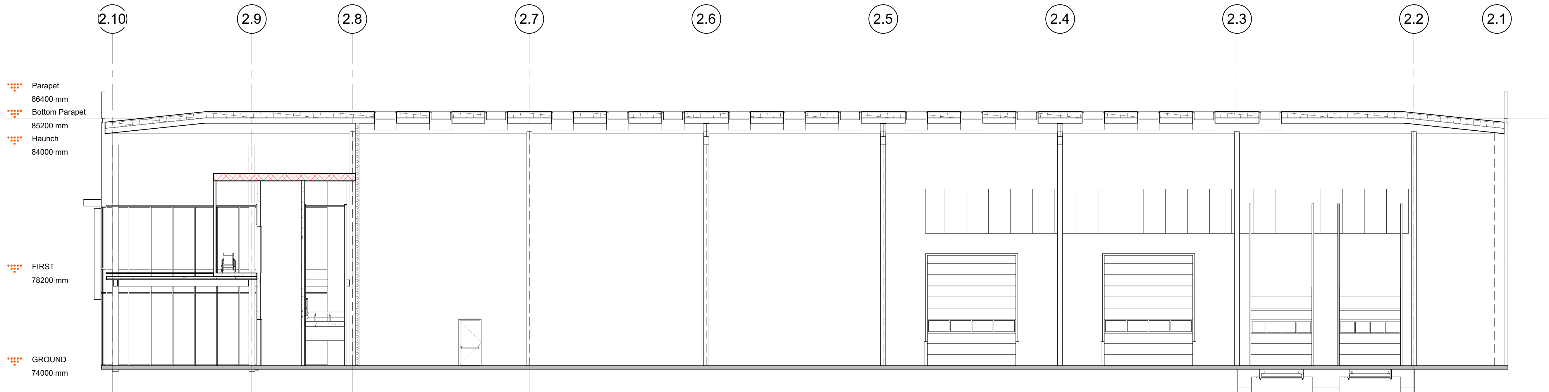
1 Warehouse Section A 1 : 100
