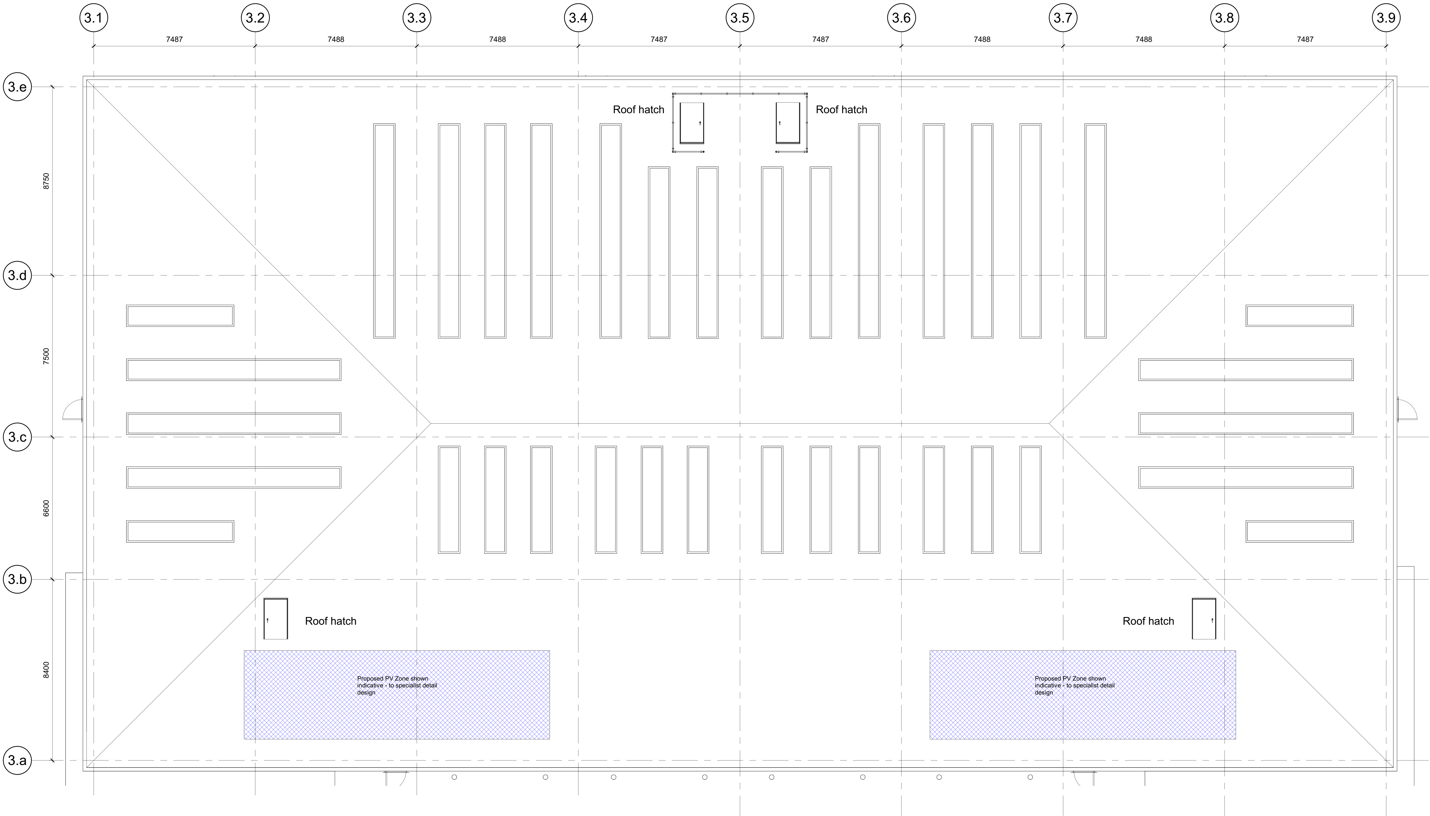
1 Roof Level GA Plan 1 : 100
