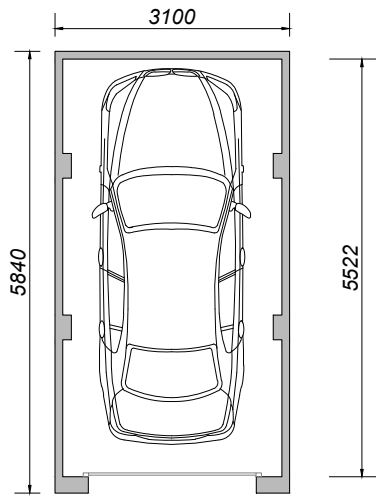
Floor Plan
