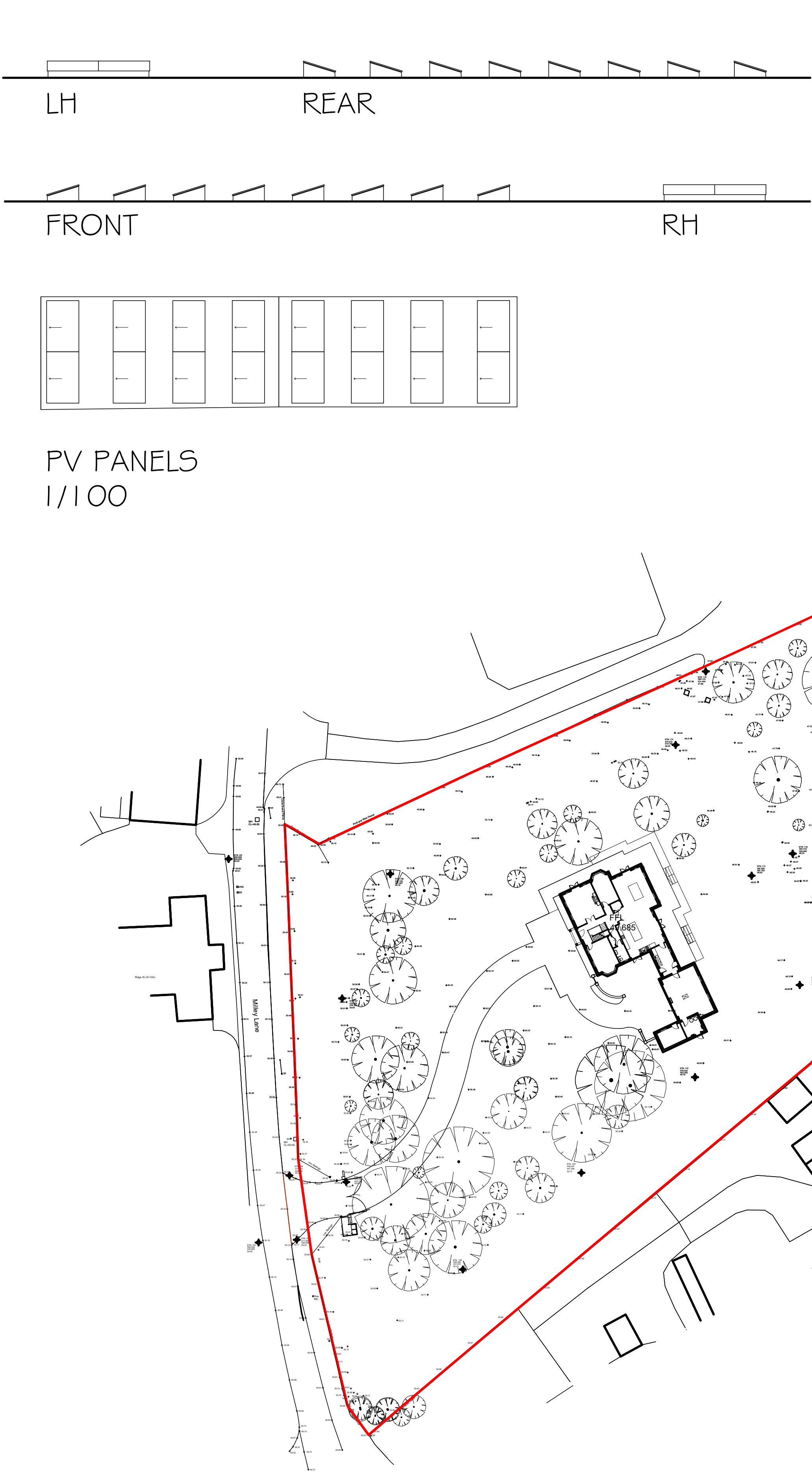
PROPOSED SITE PLAN 1/500
