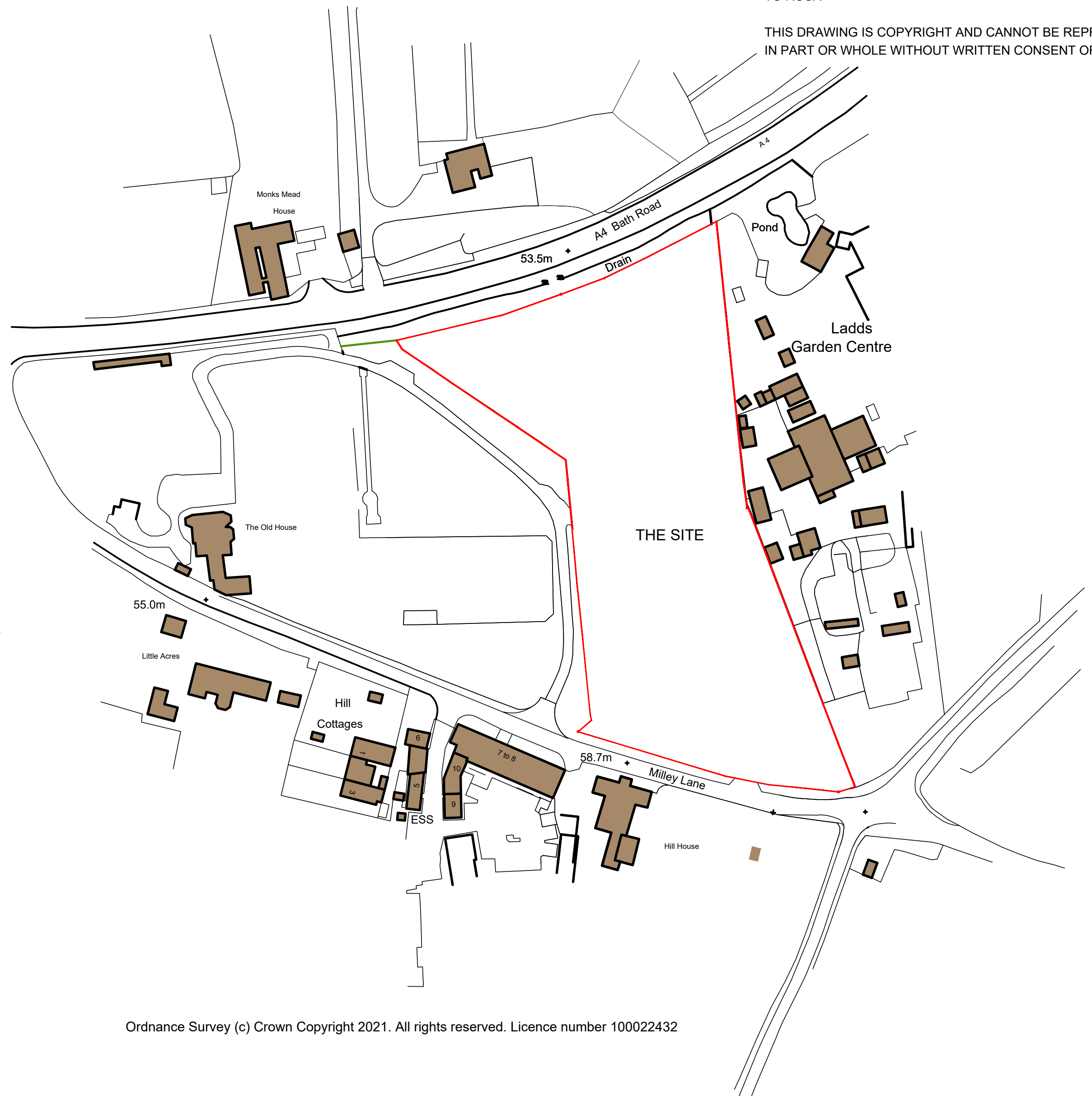
LOCATION PLAN 1/1250
