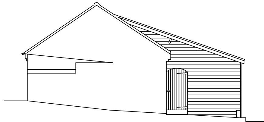
EXISTING ELEVATION 'A'.
