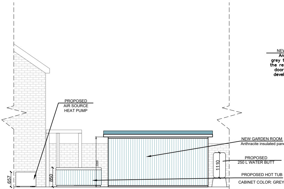
Garden Room Proposed North Elevation
