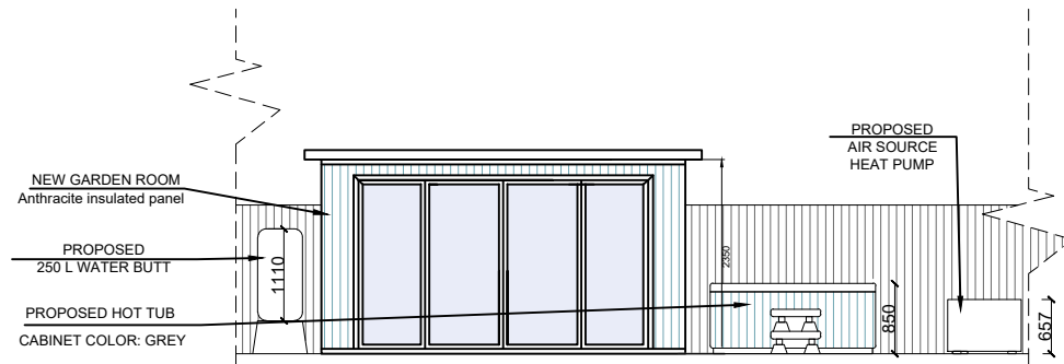
Garden Room Proposed South Elevation
