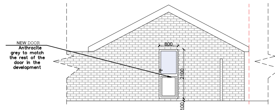
Garage Proposed East Elevation
