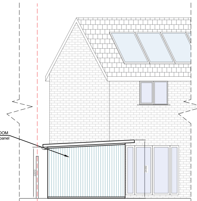
Garden Room Proposed West Elevation
