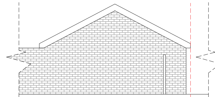
Garage Existing East Elevation
