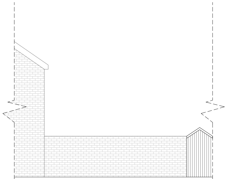
Garden Room Existing North Elevation
