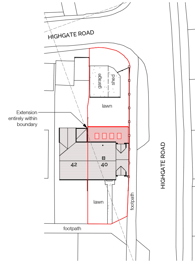
PROPOSED SITE BLOCK PLAN Scale 1 : 500
