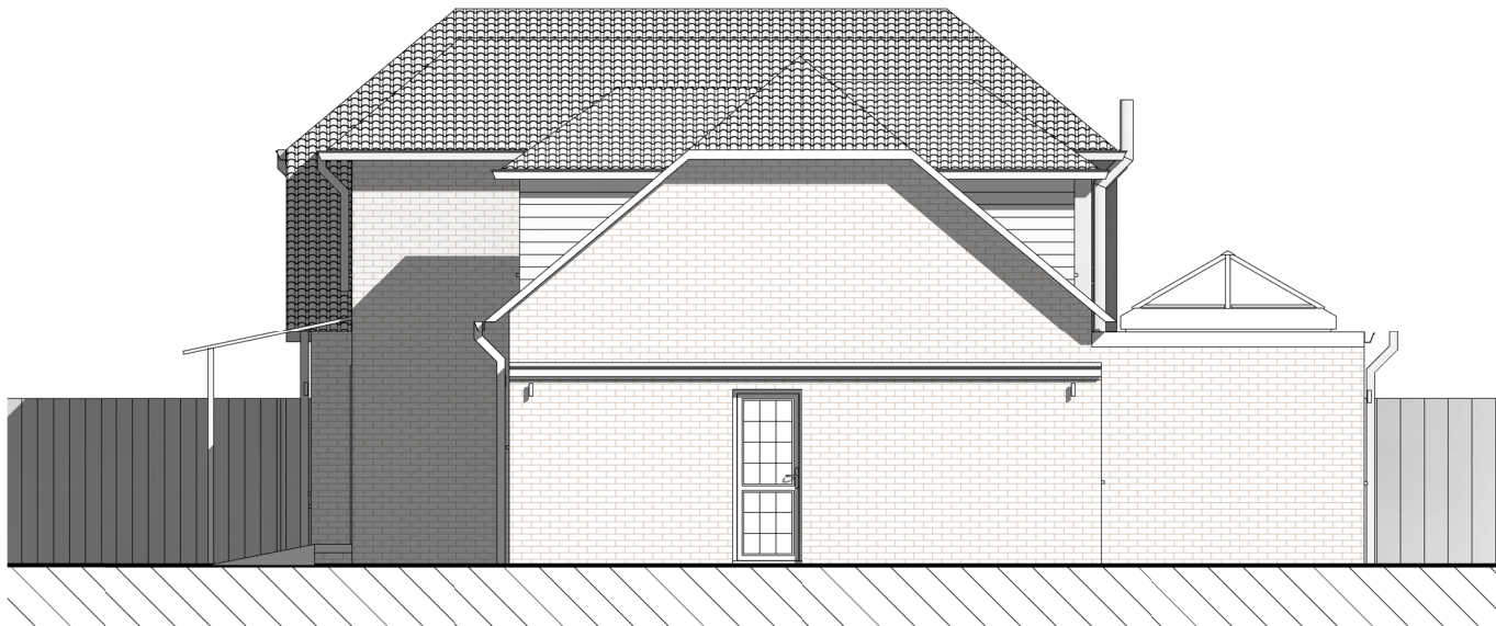
Side - North - Planning 1 : 100
