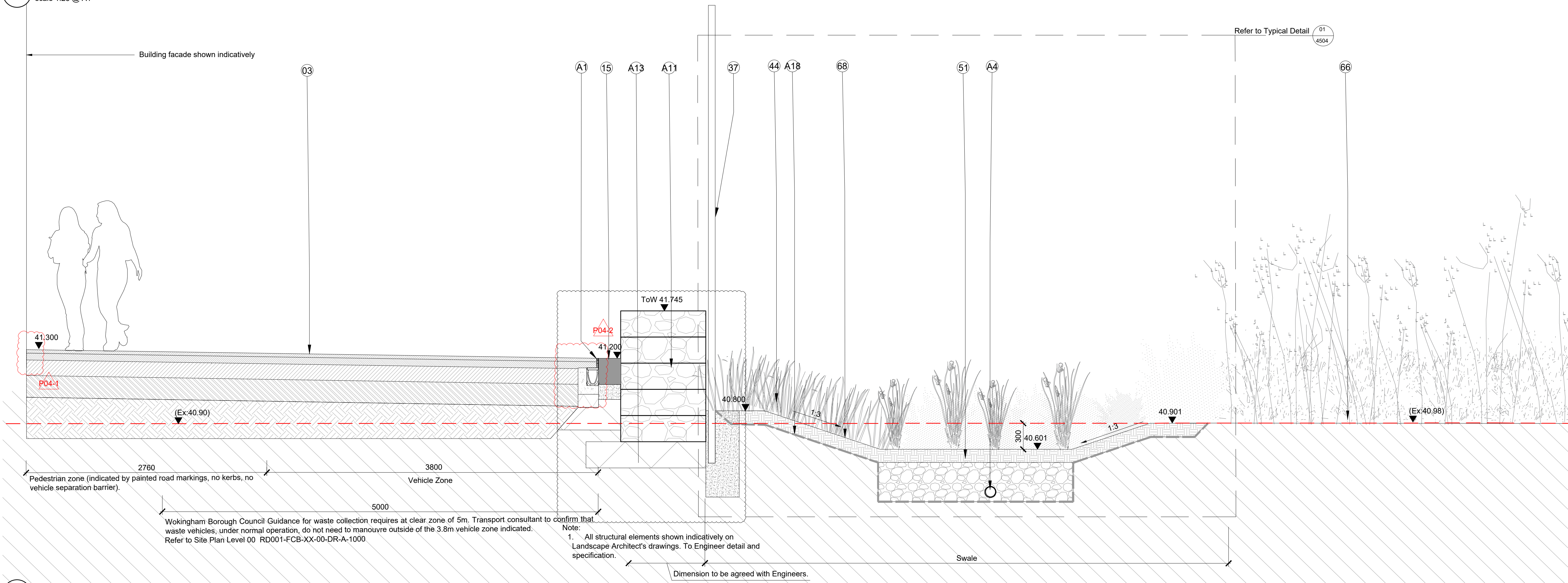
02 Section 13 - Service road and swale scale 1:25 @ A1
