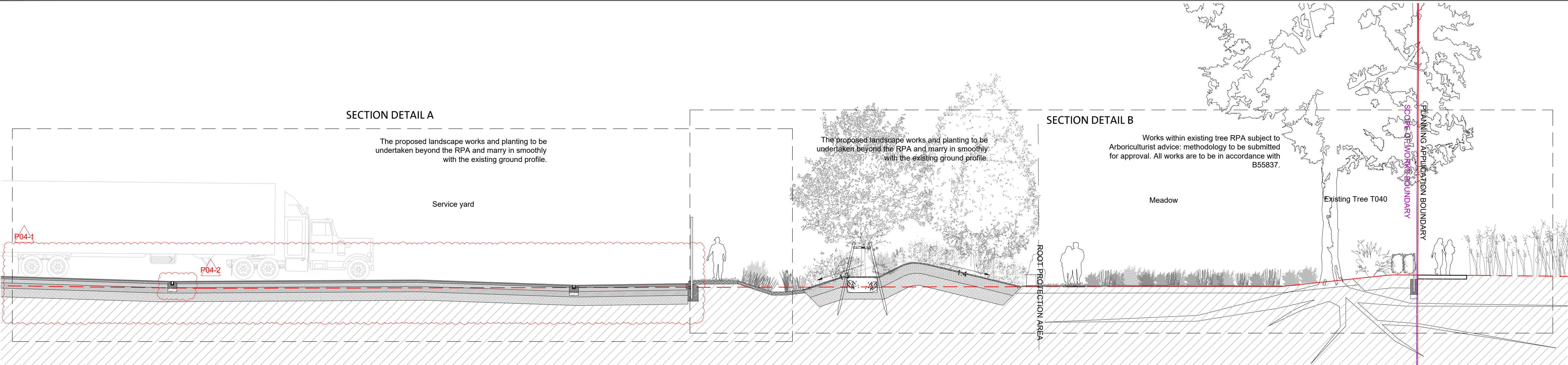
01 Section 6 - Service yard and South garden scale 1:100 @ A1
