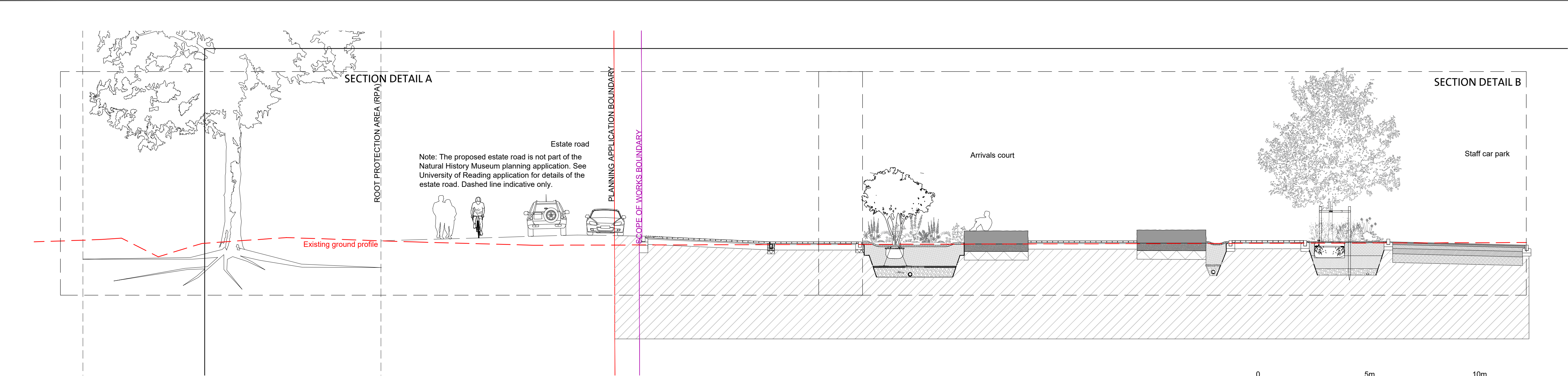
01 Section 8 - Arrival court scale 1:100 @ A1
