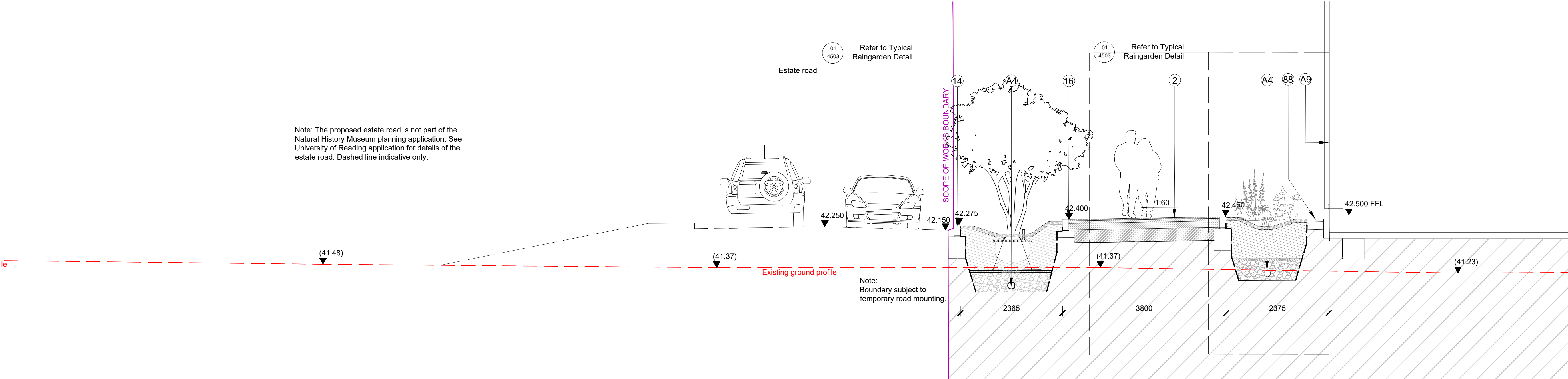
01 Section 12 - West Road scale 1:50 @ A1
