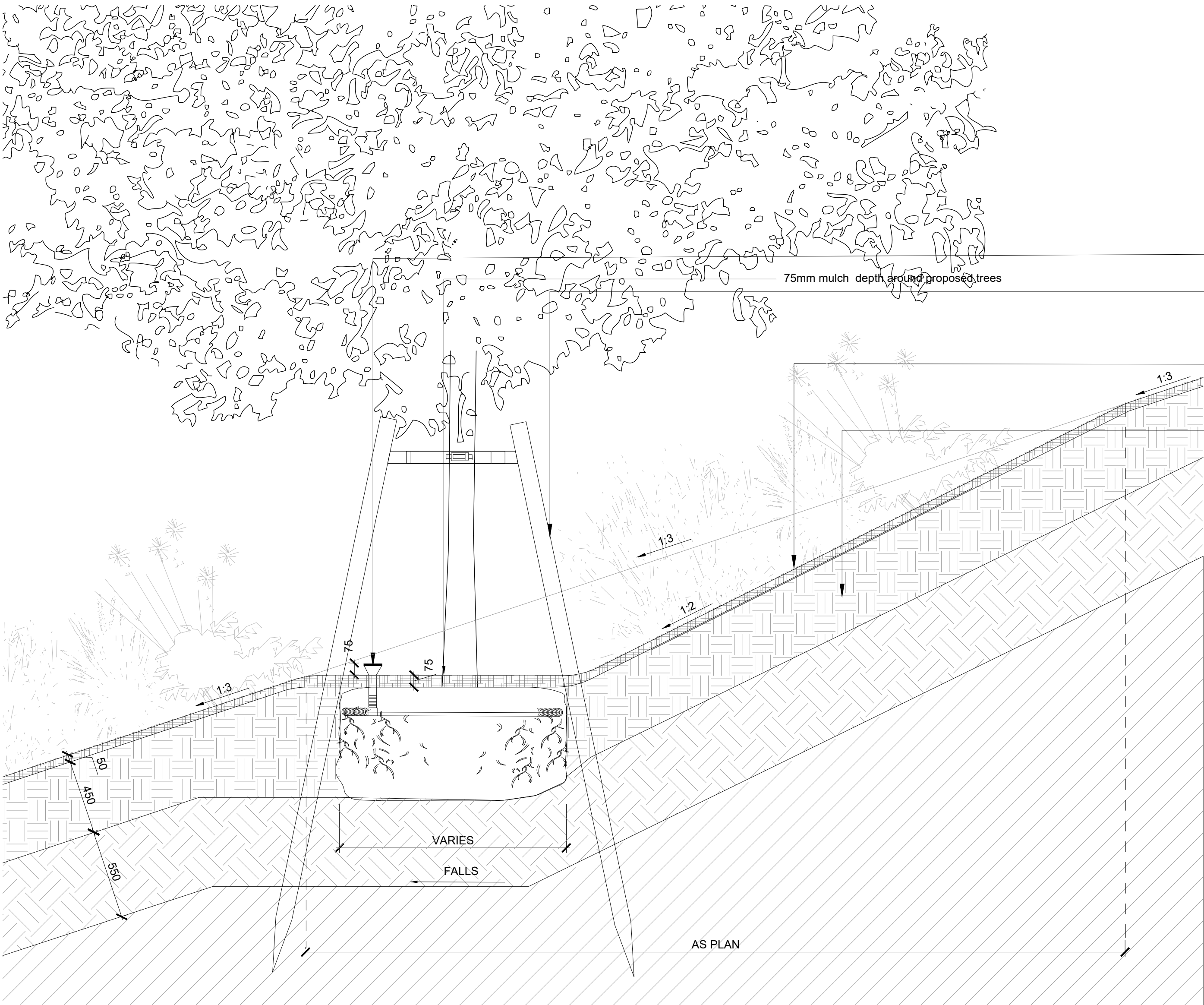
1 TYPICAL TP03 - TREE PIT IN SOFT - WOODLANDS AREA scale 1:20 @ A1
