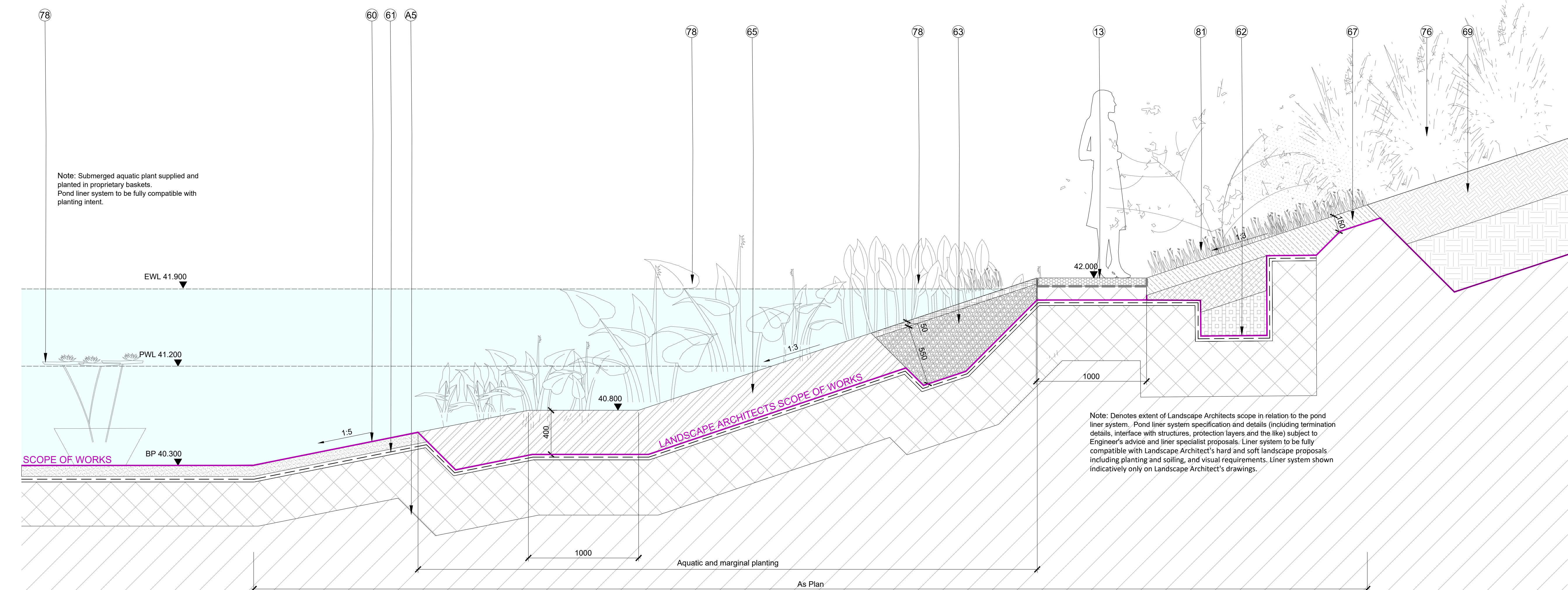
3 TYPICAL WATER POND EDGE DETAIL scale 1:20 @ A1
