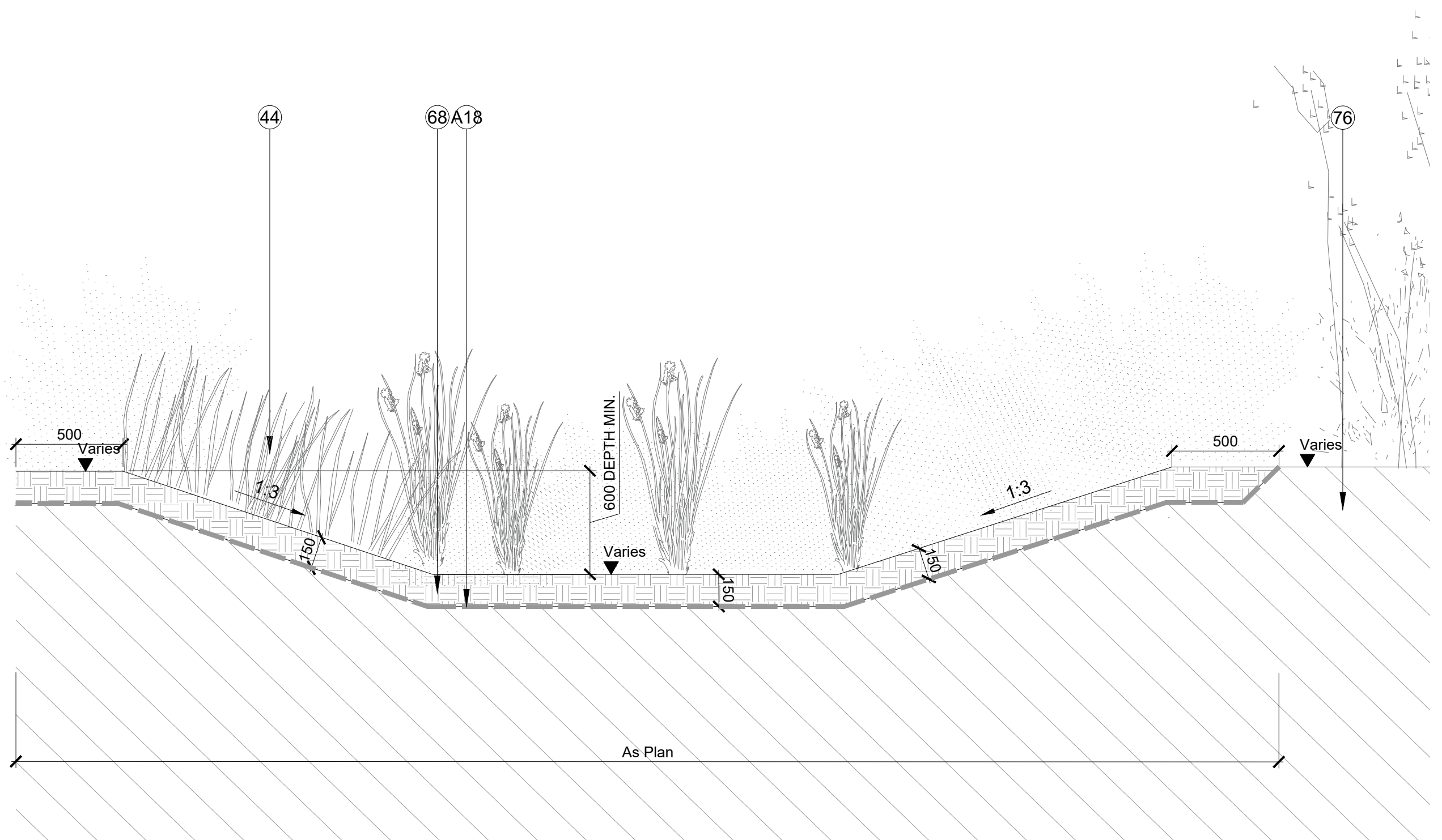
2 TYPICAL SOUTH SWALE DETAIL scale 1:20 @ A1
