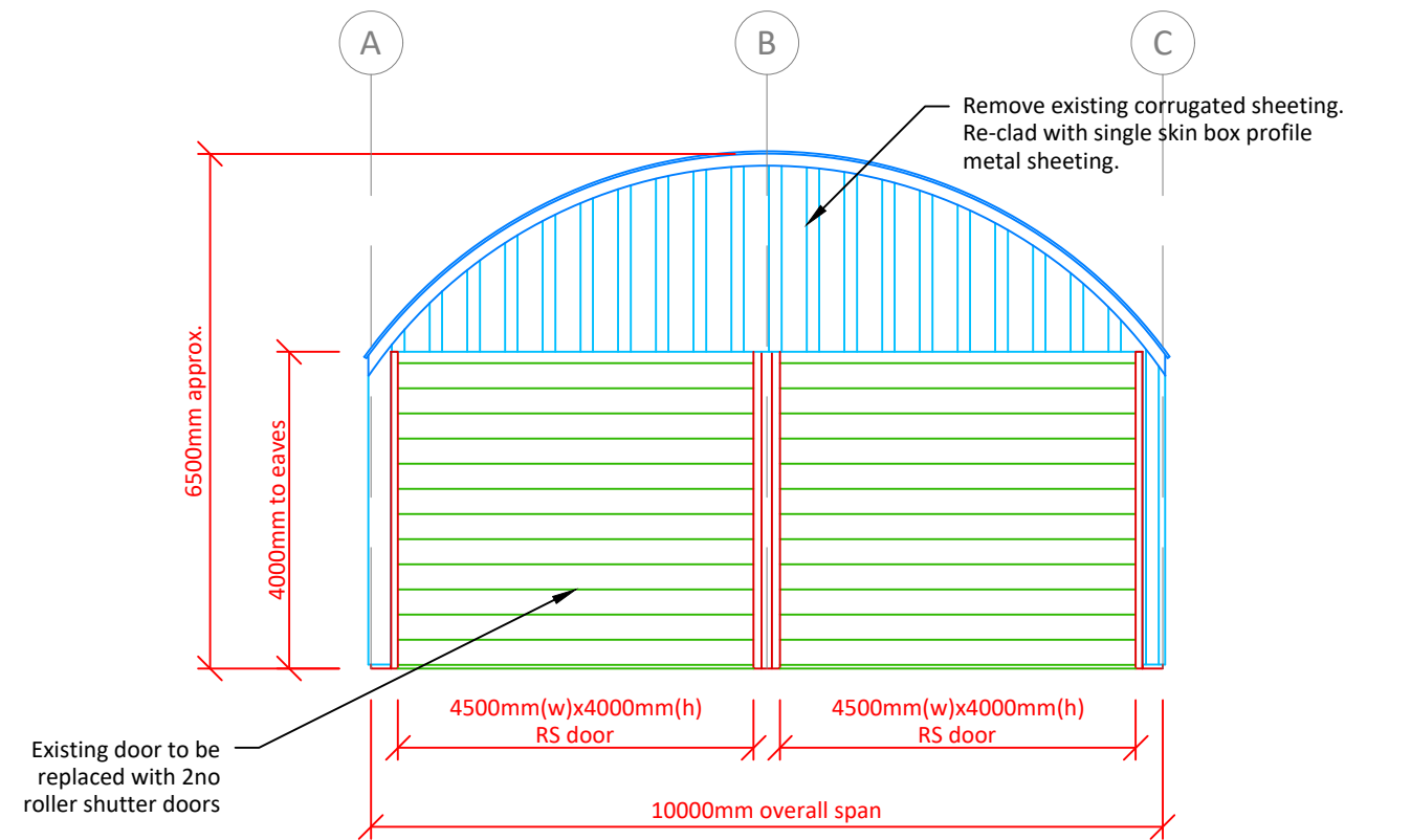
ELEVATION ACROSS GRIDLINE 1
