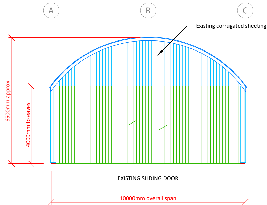
ELEVATION ACROSS GRIDLINE 1
