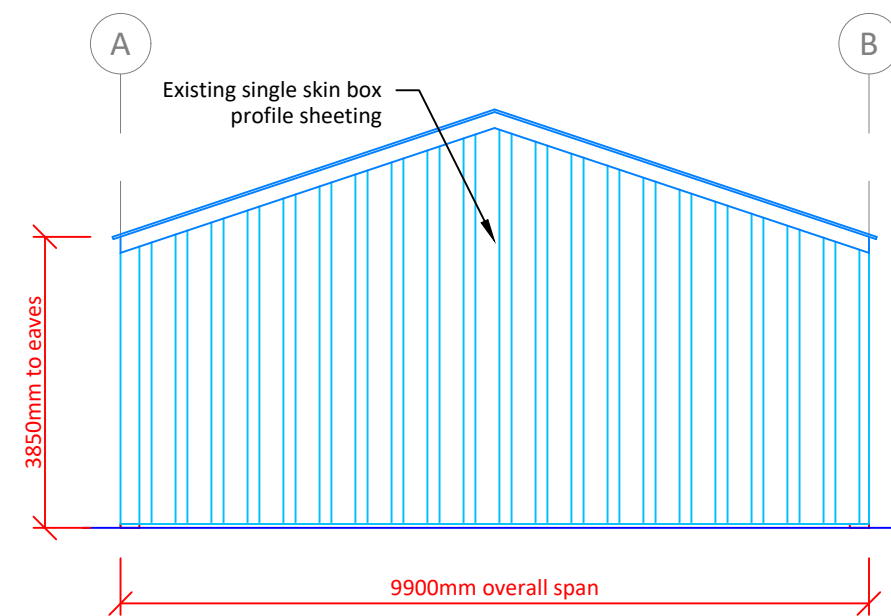
ELEVATION ACROSS GRIDLINE 1
