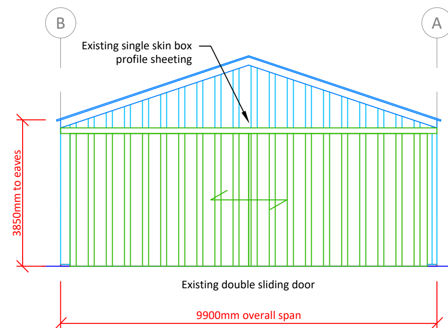
ELEVATION ACROSS GRIDLINE 10
