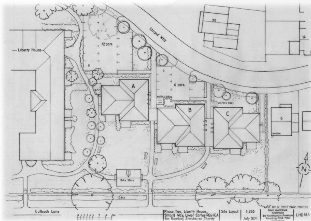
Figure 3: Proposed scheme, drawing number LHD 16A (Matt Andrews Architect)
