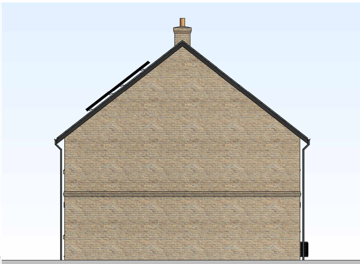
Proposed Side Elevation 2 1 : 100
