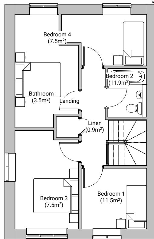
First Floor Plan 1 : 100
