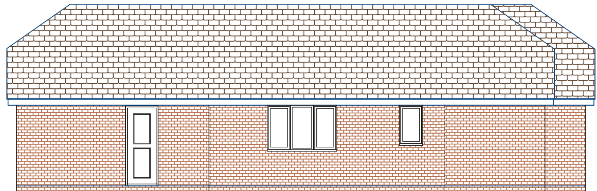
Proposed Side Elevation (L) Revised
