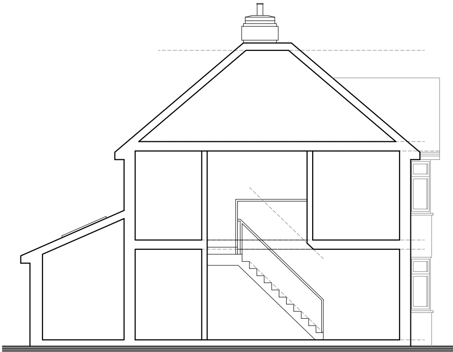
1:100 Existing Side Section
