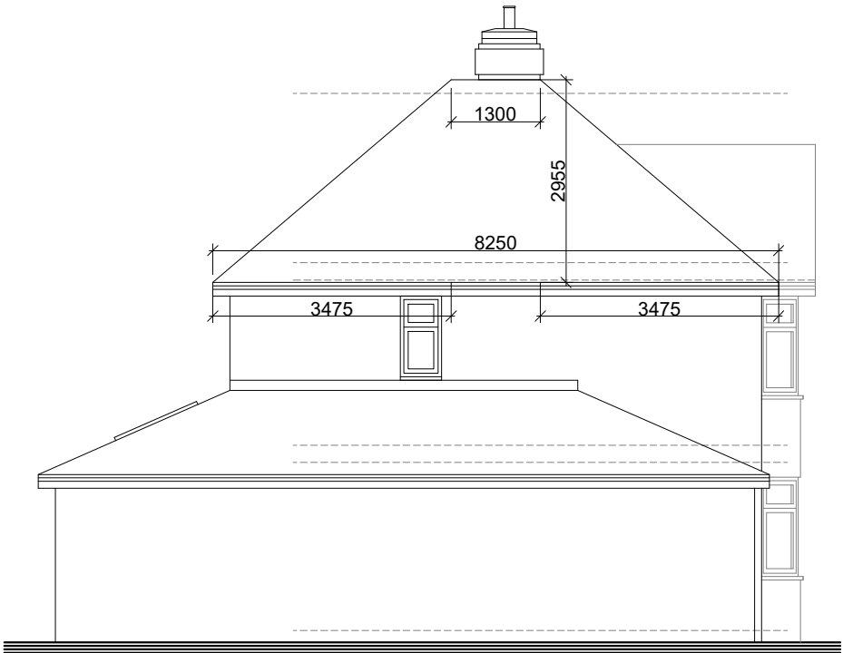
1:100 Existing Lh side Elevation
