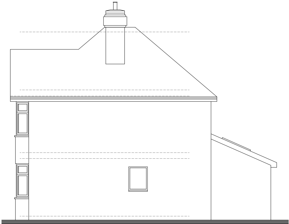
1:100 Existing Rh side Elevation
