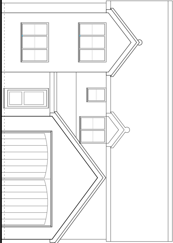
FRONT ELEVATION AS PROPOSED (NO CHANGE)
