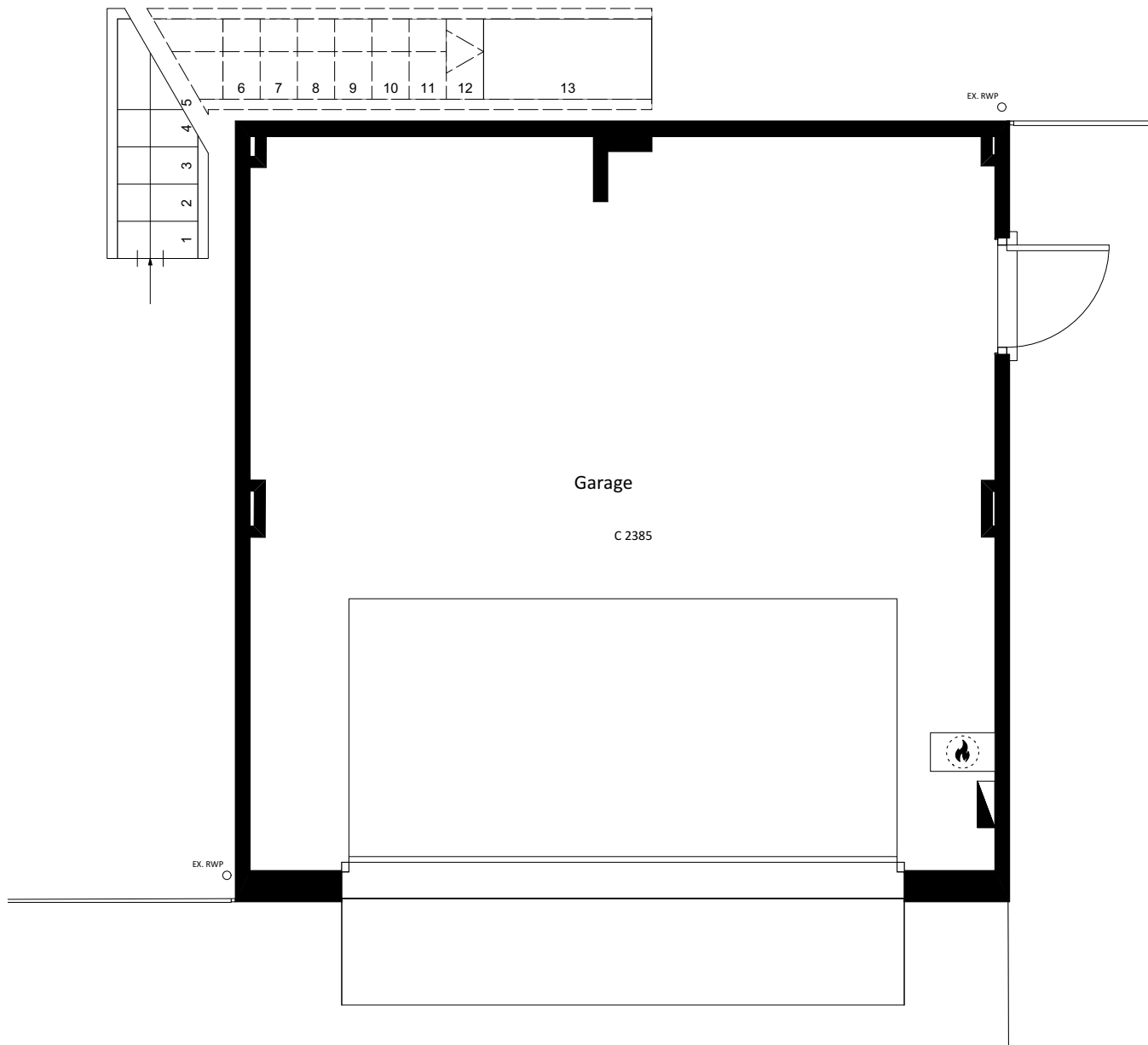
PRO Ground Floor Plan - As Existing
