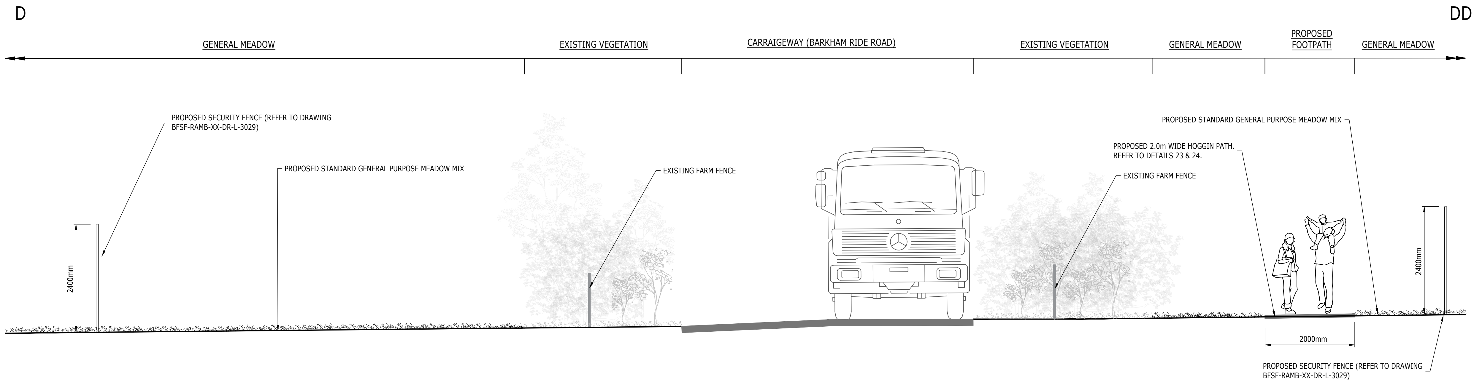
04 BARKHAM RIDE ROAD SECTION NOT TO SCALE
