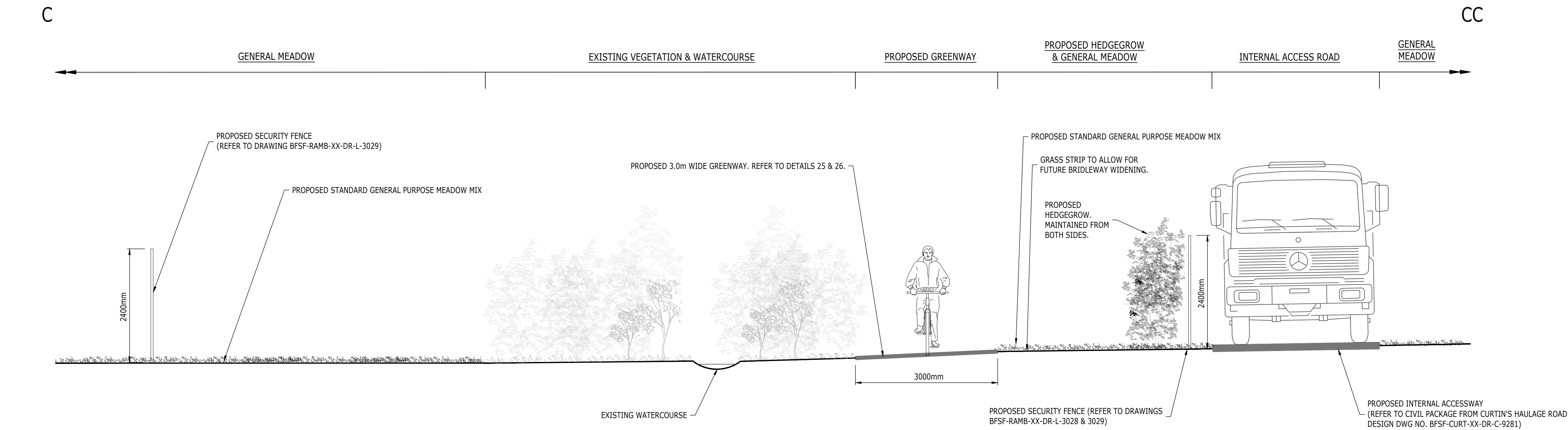
03 PROPOSED GREENWAY & INTERNAL SITE ACCESSWAY SECTION NOT TO SCALE
