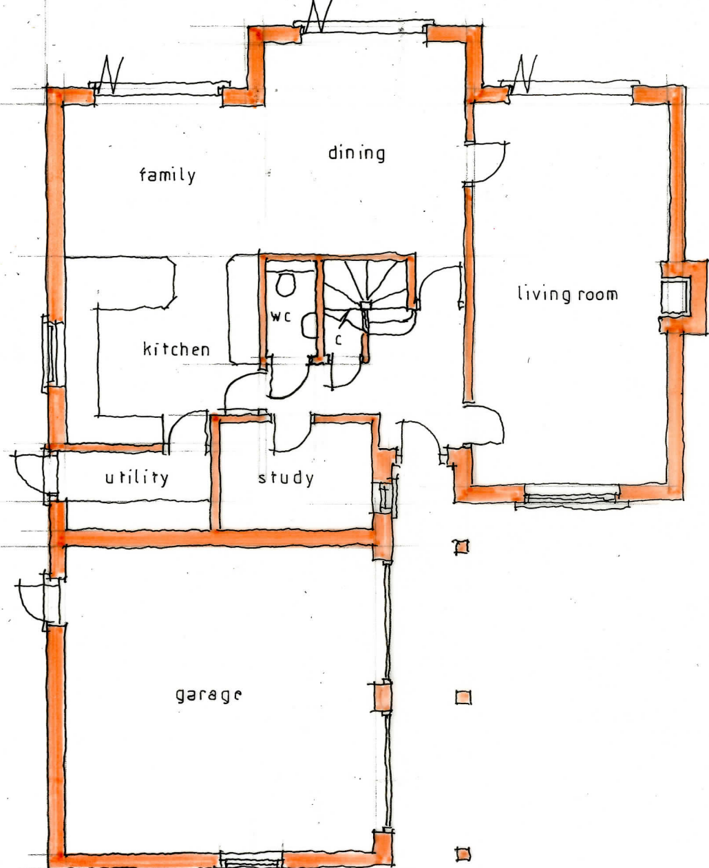
GROUND FLOOR
