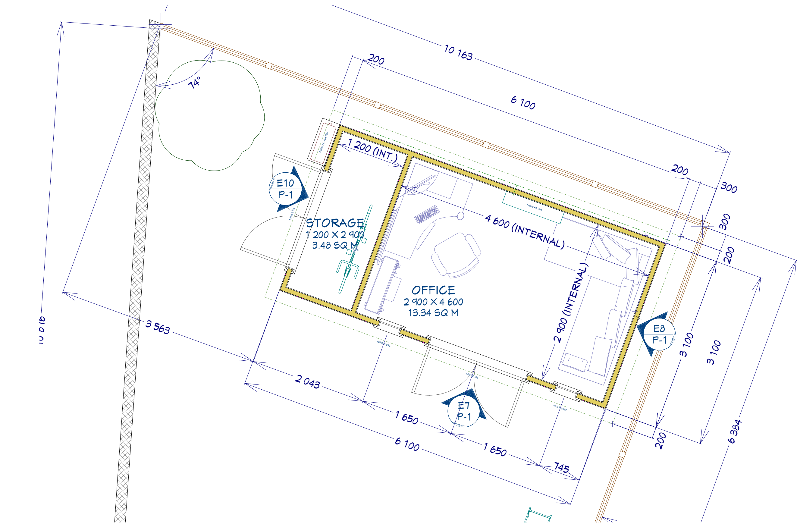
Outbuilding Plan
