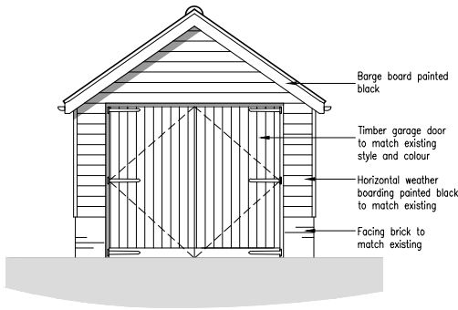
Front Elevation
