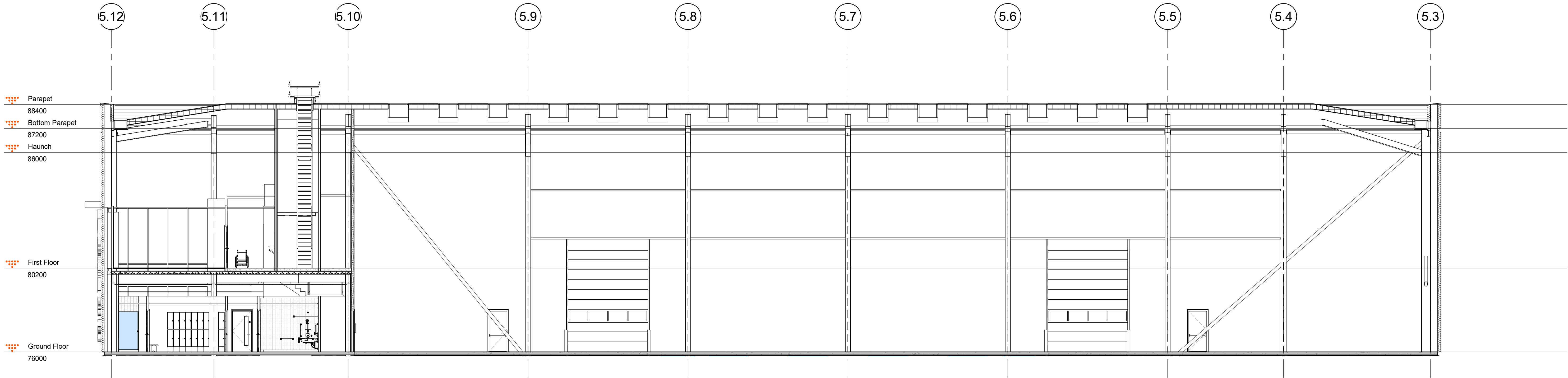
1 WAREHOUSE SECTION A 1 : 100
