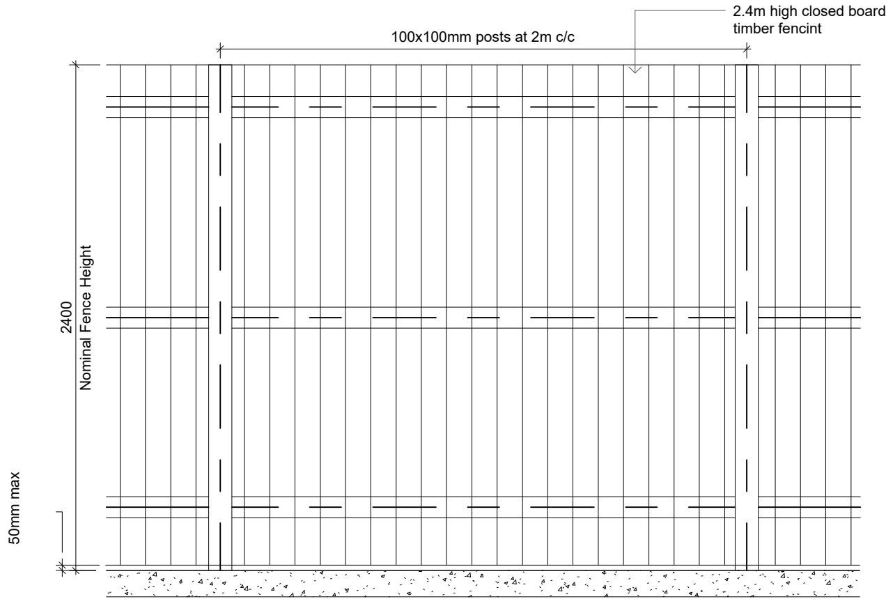
2400mm High Plant Compound Fence Elevation (Internal face)
