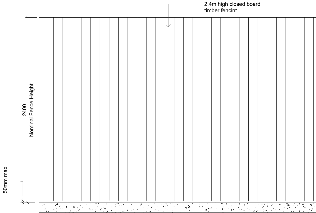
2400mm High Plant Compound Fence Elevation (External face)
