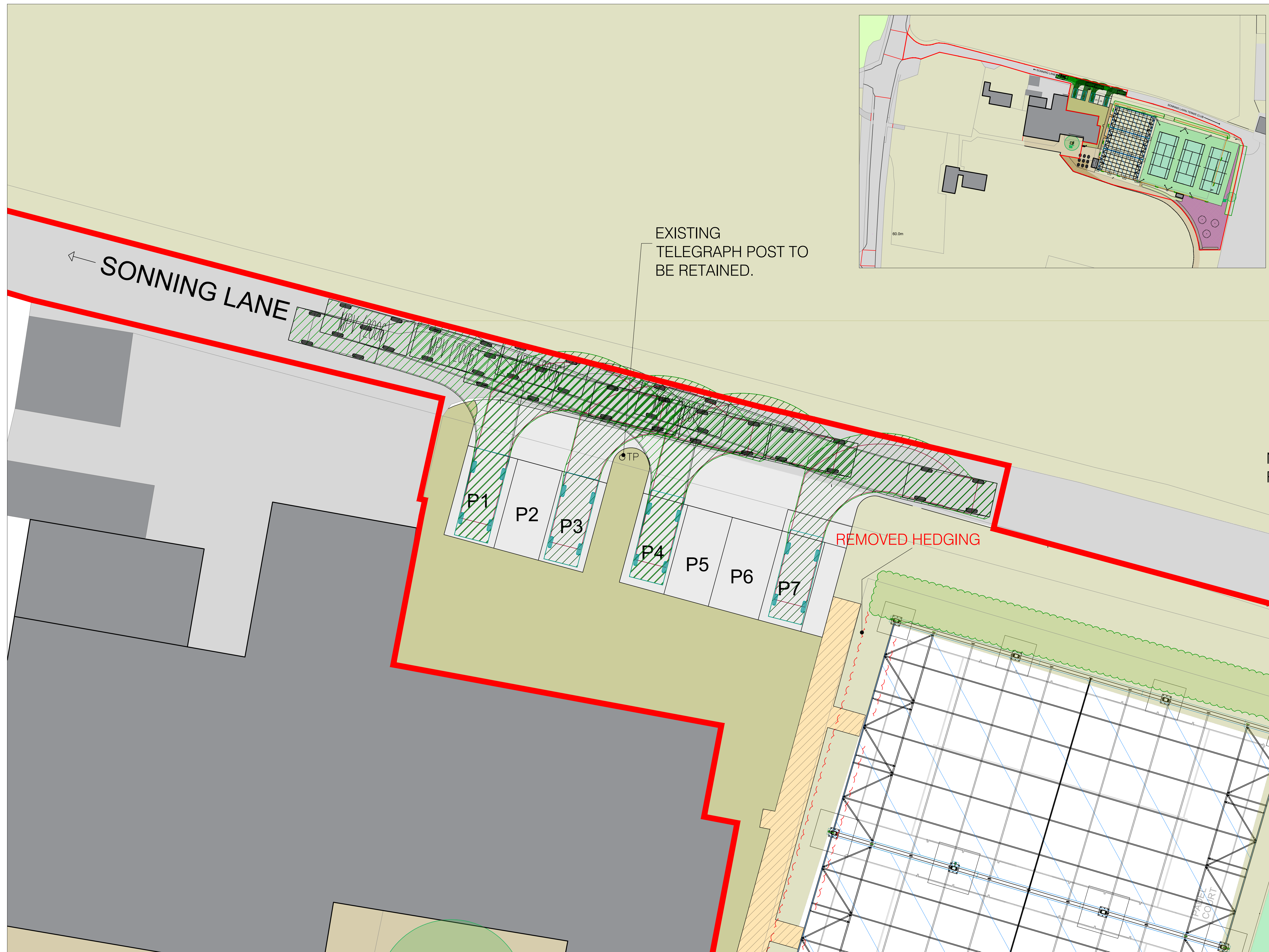
PARKING LAYOUT
