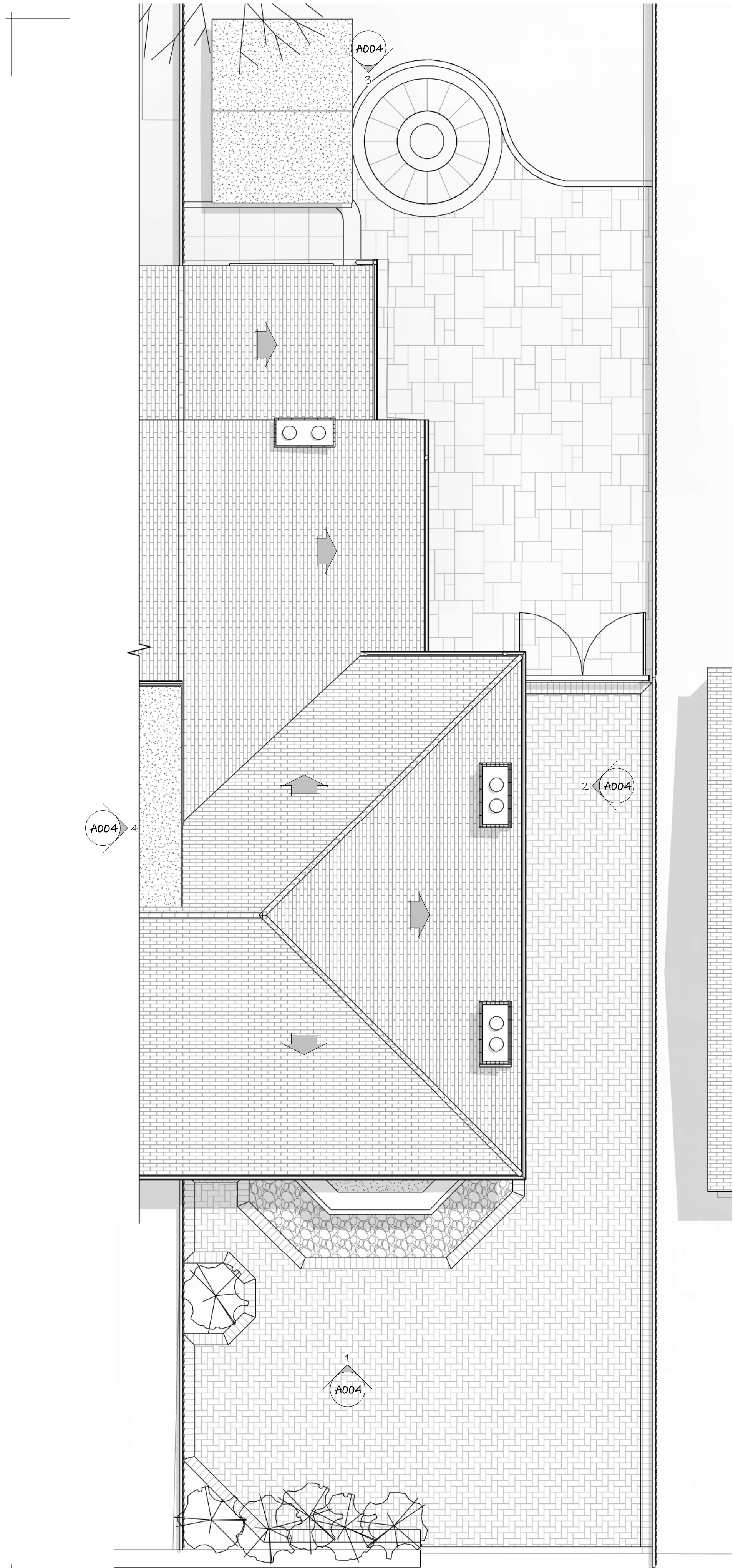
1 Existing Roof 1:50
